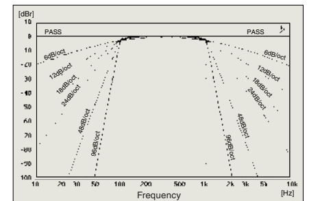
Fig. 2 Divider unit slope characteristics (bandpass filter) [Cutoff frequency setting 100 Hz for lower and 1 kHz for upper range]
