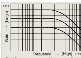
Fig. 4 Frequency response with current feedback (Response remains uniform also when gain changes)
